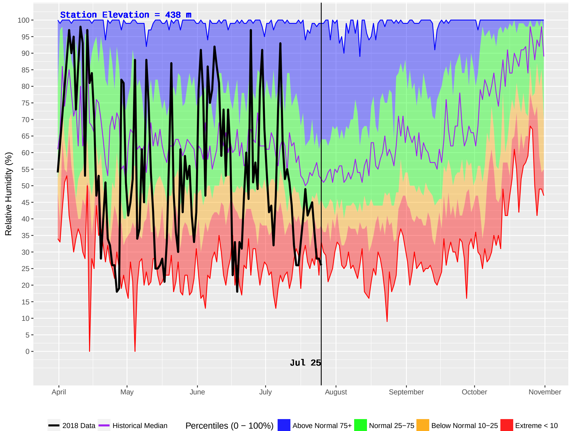
MENZIES CAMP (19) : Historical (1970–2016) and Current (2018) Noon Relative Humidity
